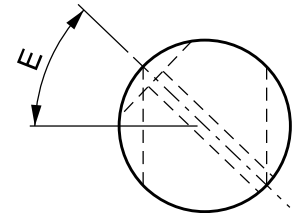
View on A-A Orientation of scarfing for strut pole
